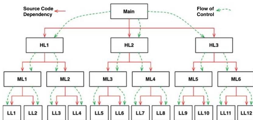
Figure 5.1 Source code dependencies versus flow of control
